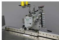
伺服电机传输自动入料 Servo motor driven and automatic feeding
