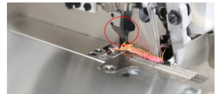
砍刀剪线装置将前工序的线头和缝纫结束后的线头控制在 5mm 以内, 免去二次剪线头的烦恼; The thread end of the previous process and the thread end after sewing can be controlled within 5mm, eliminating the trouble of secondary thread end trimming
